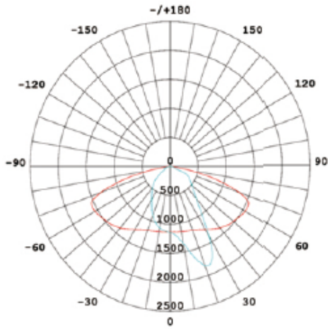
T2S5882 / T2S5892 (M7A-9 / M7A-18) IESNA Type II Short
