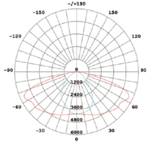
T1S2841 / T1S2861 (M7A-24 / M7A-36) IESNA Type I Short
