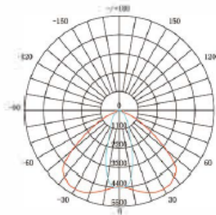
11D3030 Beam Angle (50%) 110×40DEG
