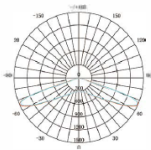
T5S3040 IESNA Type VS Short
